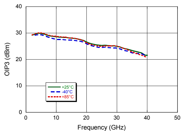
Output IP3
