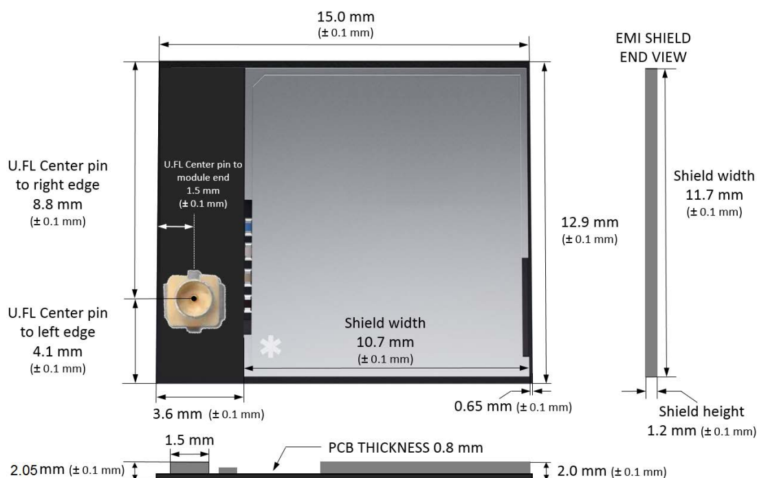
Figure 9.2. BGM13P with U.FL Package Dimensions
