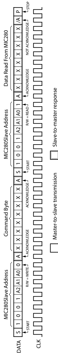
Figure 2. READ_BYTE Protocol
