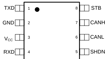
TCAN334 D, DCN Packages 8-Pin SOIC, SOT-23 Top View
