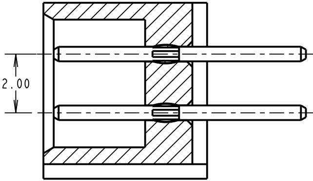
SECTION X-X
