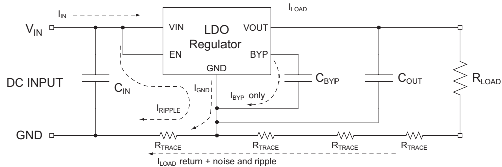
Figure 2: Recommended LDO Regulator Layout.
