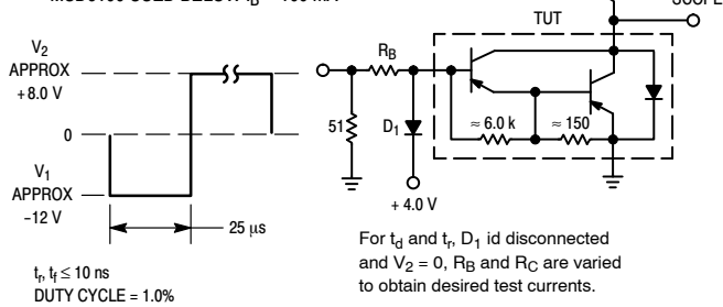
Figure 2. Switching Times Test Circuit
