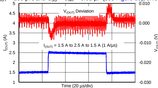
Figure 13. LOAD TRANSIENT RESPONSE
