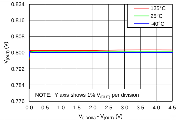
Figure 3. LDOIN LINE REGULATION
