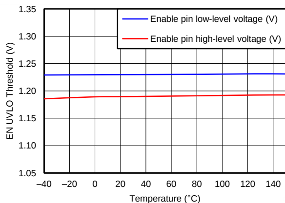
Figure 17. DC-DC EN UVLO THRESHOLD vs TEMPERATURE
