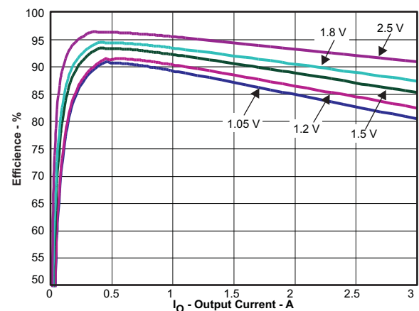
Figure 24. DC-DC Efficiency vs Output Current
