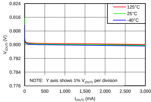
Figure 1. LOAD REGULATION
