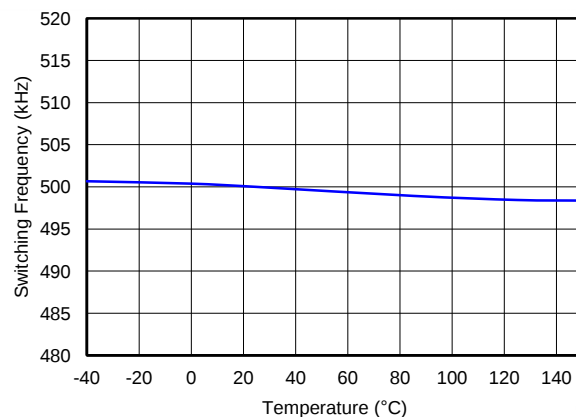
Figure 16. DC-DC SWITCHING FREQUENCY vs TEMPERATURE
