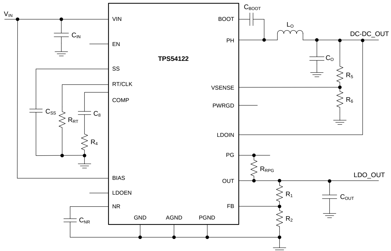
Figure 25. Typical Application
