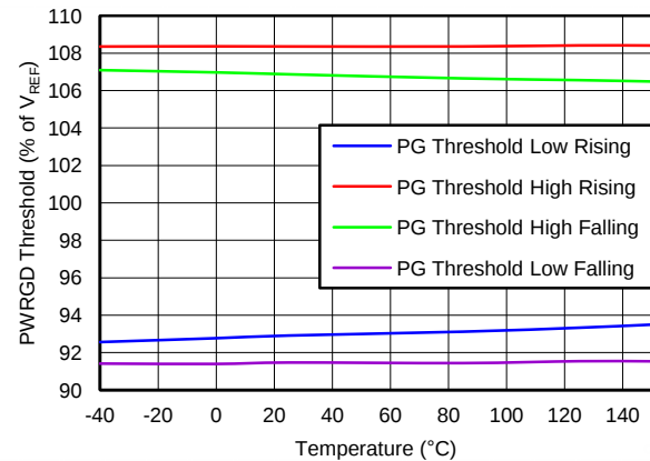
Figure 20. PG THRESHOLD vs TEMPERATURE
