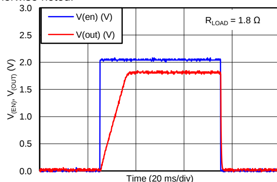
Figure 14. ENABLE PULSE RESPONSE
