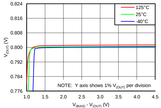
Figure 4. LDO BIAS LINE REGULATION
