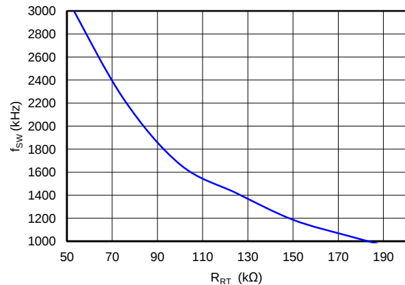
Figure 22. DC-DC SWITCHING FREQUENCY vs R_{RT}
