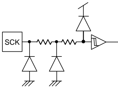
Figure 53. SCK input equivalent circuit
