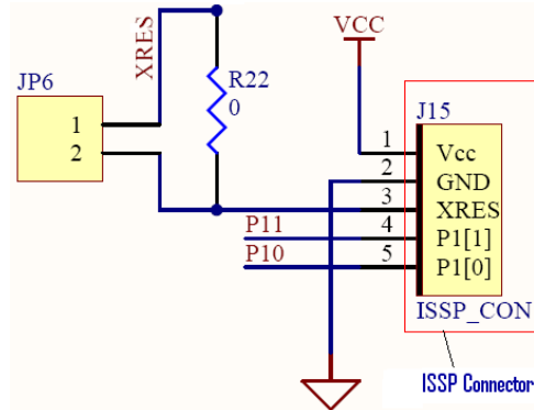
Figure 4-10. ISSP Connector
