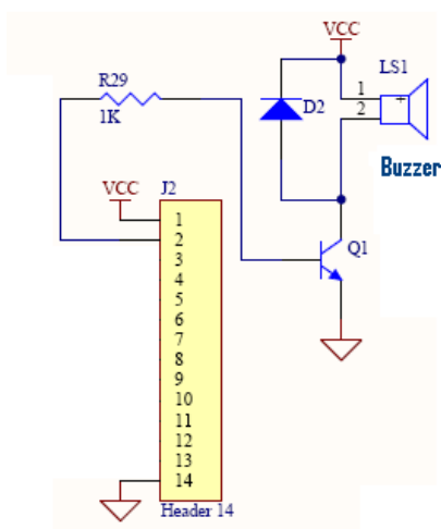
Figure 4-9. Buzzer
