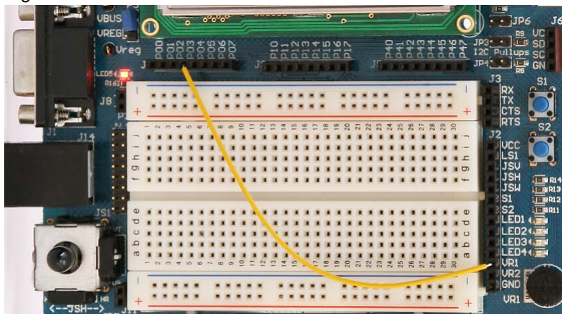
Figure 5-49. Hardware Connection
