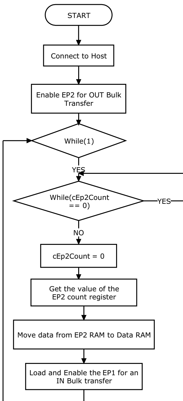
Figure 5-65. Flowchart
