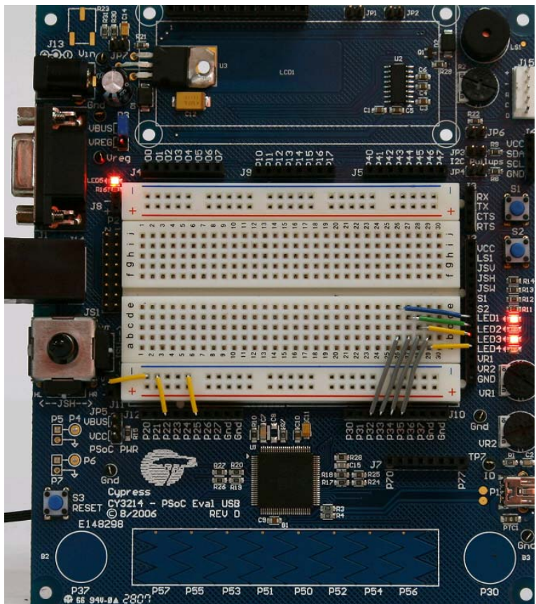
Figure 5-38. Hardware Connection
