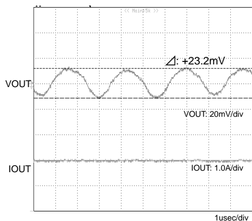
Fig.16 Output Ripple Voltage ( V_{IN} = 12V V_{OUT} = 3.3V L = 10\mu H C_{out} = 22\mu F I_{out} = 2.0A )
