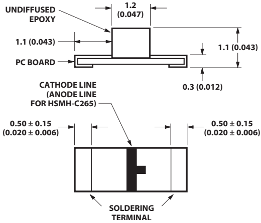
HSMx-C265
