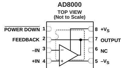
Figure 1. 8-Lead AD8000 , 3 mm x 3 mm LFCSP (CP-8-13)
