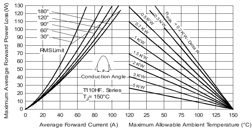
Fig. 21 - Forward Power Loss Characteristics
