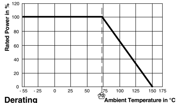
Derating
