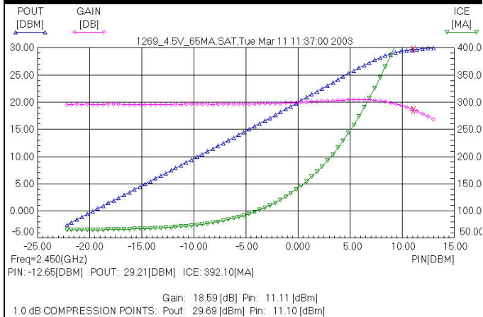
Figure 7 – Power Sweep (Vc = 4.5V, Vref = 2.85V, Icq = 65mA)
