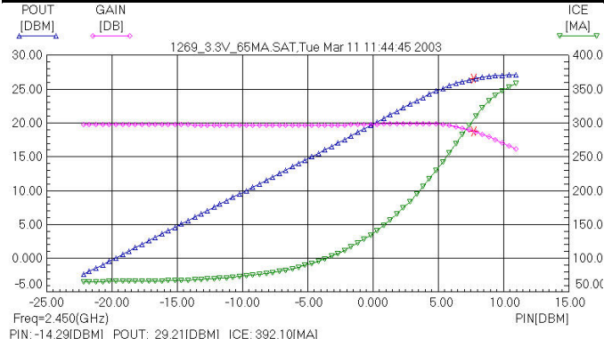
Gain: 18.77 [dB] Pin: 7.75 [dBm] 1.0 dB COMPRESSION POINTS: Pout: 26.52 [dBm] Pin: 7.75 [dBm] Figure 2 – Power Sweep (Vc = 3.3V, Vref = 2.85V, Icq = 65mA)
