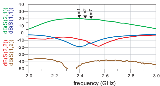
Figure 6 – S-Parameter Data (Vc = 4.5V, Vref = 2.85V, Icq = 65mA)
