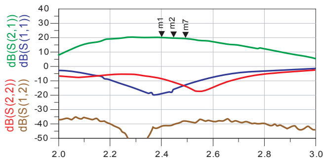
Figure 1 – S-Parameter Data (Vc = 3.3V, Vref = 2.85V, Icq = 65mA)
