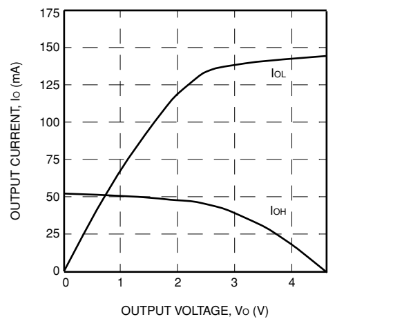
Figure 82. Fast ( T_J = 125^\circ\text{C} , V_{DD} = 4.5\text{ V} )
