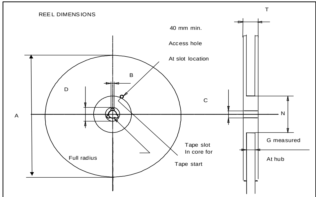
Figure 24: Reel outline
