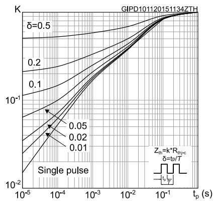
Figure 3: Thermal impedance
