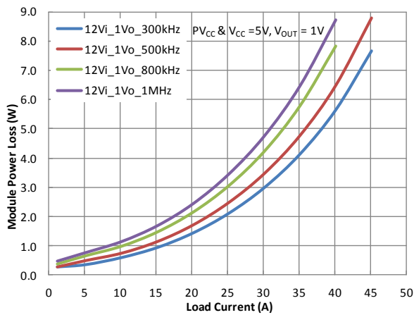
Figure 6. Power Loss vs. Output Current with 12 V IN
