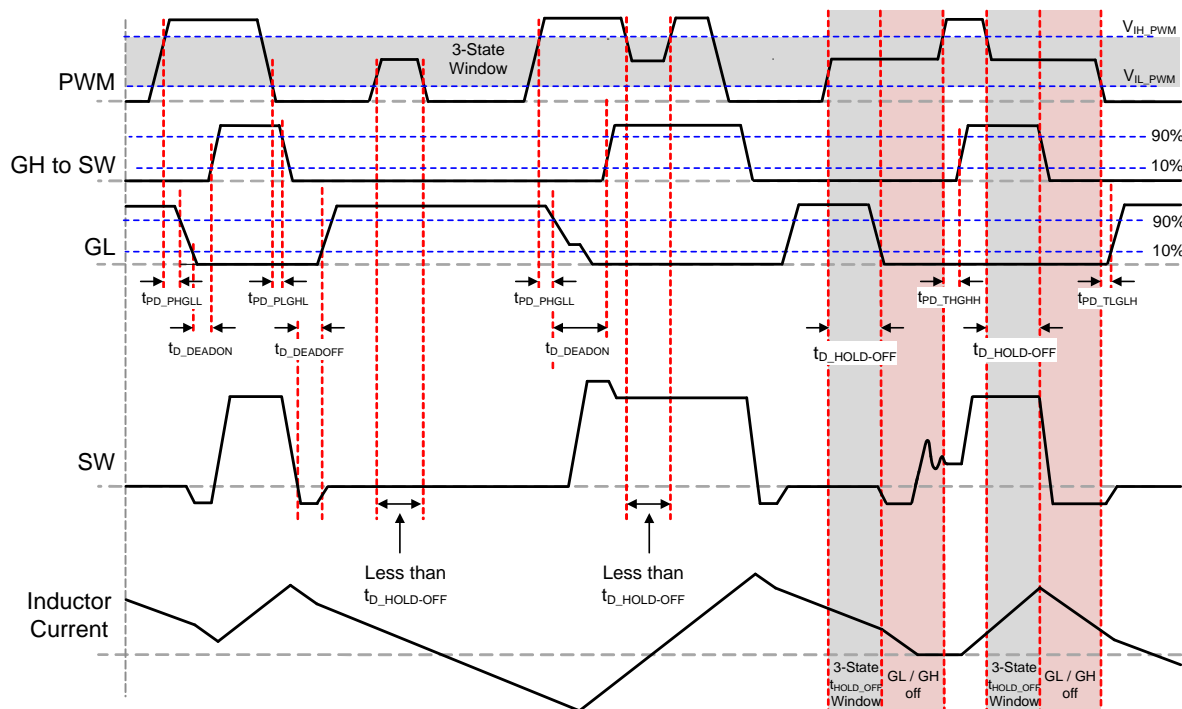
Figure 27. PWM 3-State Timing Diagram (FCCM held HIGH)
