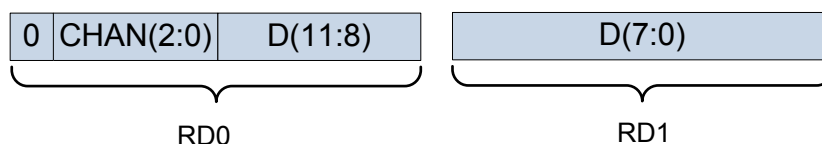
Figure 57 – Channel Data Format
