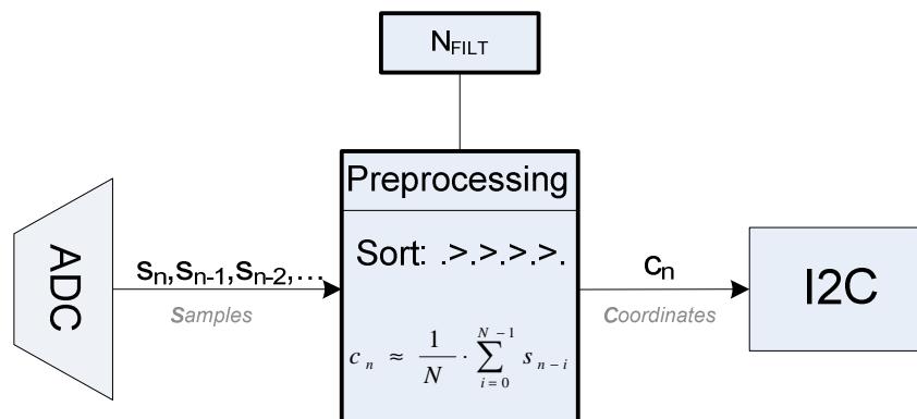
Figure 18 – Digital Processing Block Diagram
