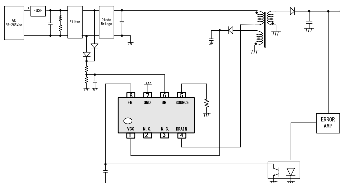
Figure 16(a). AC voltage monitor setting
