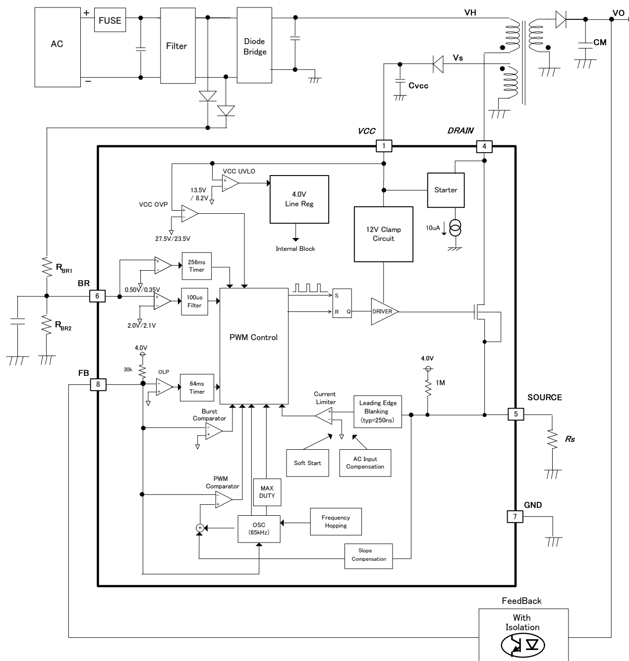
Figure 3. Block Diagram
