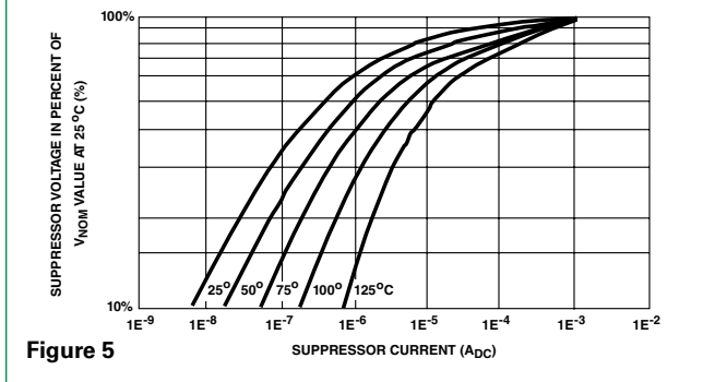
Typical Temperature Dependence of the Characteristic Curve in the Leakage Region
