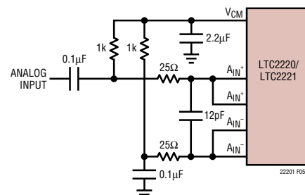
Figure 5. Single-Ended Drive
