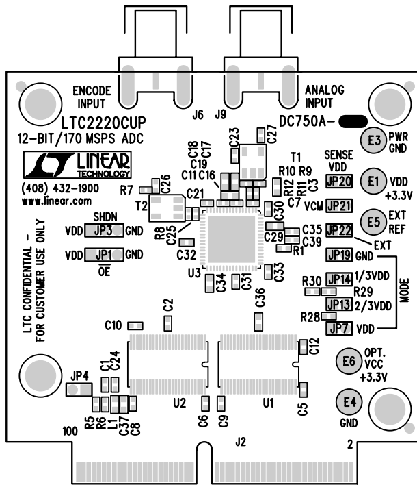
Silkscreen Top
