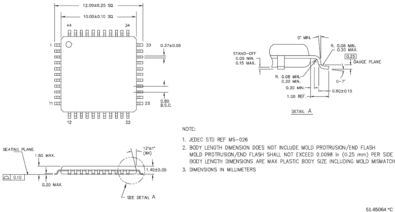
Figure 4-7. 44-Lead TQFP
