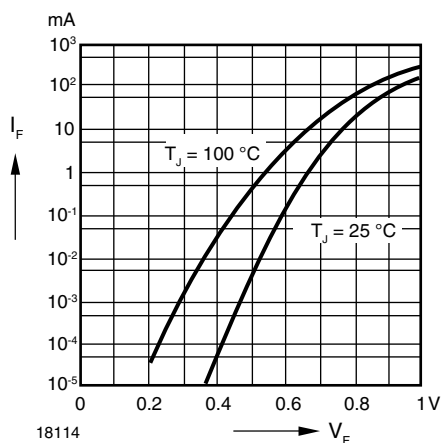
Fig. 1 - Forward Characteristics
