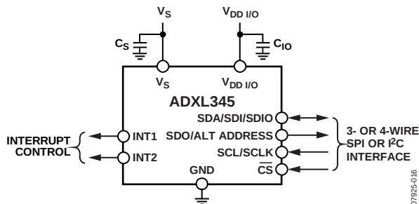
Figure 44. Application Diagram
