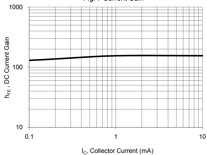
Fig. 7 Current Gain
