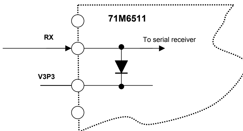
Figure 2-16: Internal Diode Clamp on the RX Pin
