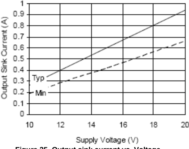
Figure 25. Output sink current vs. Voltage
