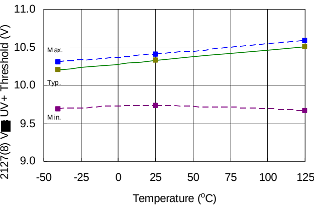
Figure 23A. 2127(8) V_{BS} UV threshold + vs. Temperature
