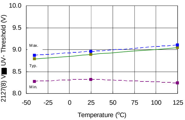
Figure 23B. 2127(8) V_{BS} UV threshold - vs. Temperature
