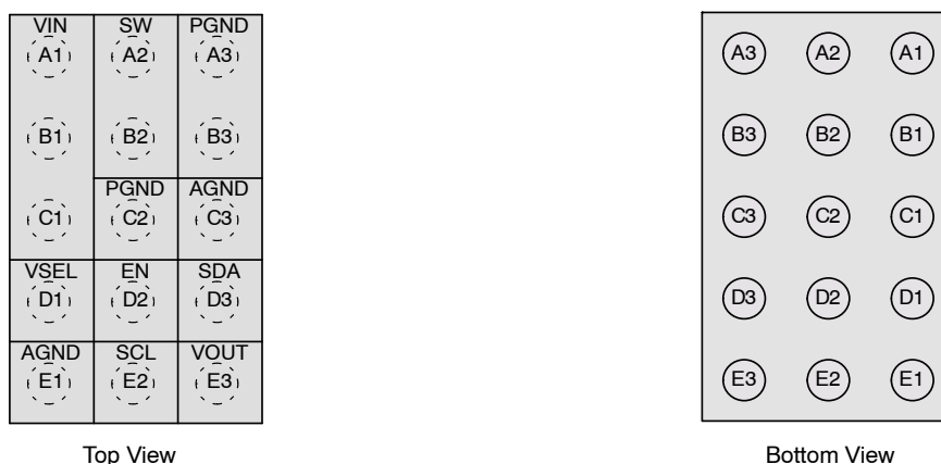
Figure 2. Pin Configuration
