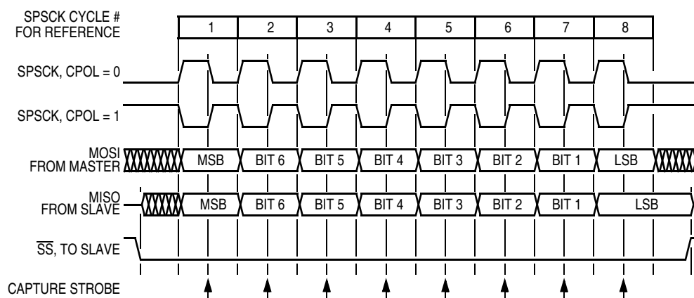
Figure 15-7. Transmission Format ( \text{CPHA} = 1 )
