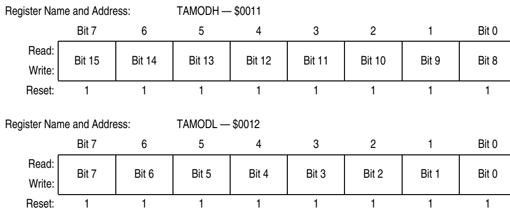
Figure 16-7. TIMA Counter Modulo Registers (TAMODH and TAMODL)
