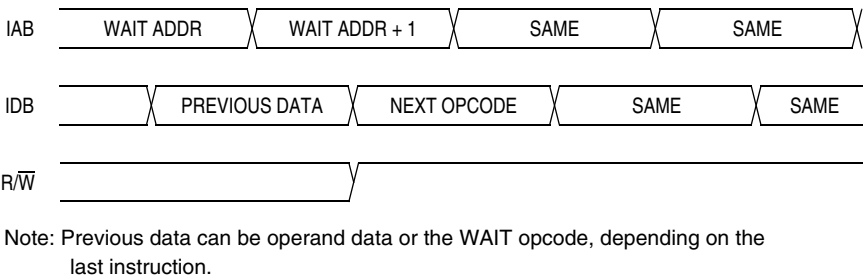
Figure 14-11. Wait Mode Entry Timing
