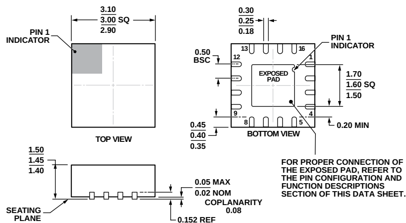
Figure 18. 16-Lead Lead Frame Chip Scale Package [LFCSP_LQ] 3 mm × 3 mm Body, Thick Quad (CP-16-28) Dimensions shown in millimeters
