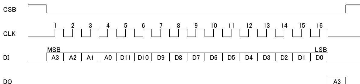
Figure 12. Communication Format
