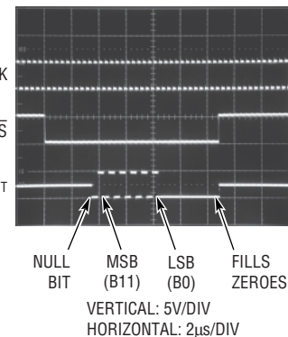
Figure 24. Scope Trace of the LTC1294/6 “Quick Look” Circuit Showing A/D Output 1010101010 (AAA HEX )
