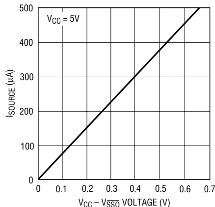
LTC1296 SS O Source Current vs V_{CC} - V_{SSO}
