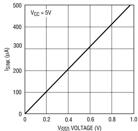
LTC1296 SS O Sink Current vs V_{SSO}
