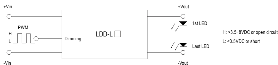
Fig-1 12VDC input, 1~3 LEDs(Vf=3V)
