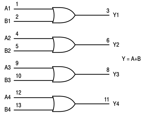
LOGIC DIAGRAM
