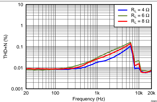
Figure 15. THD+N vs Frequency
