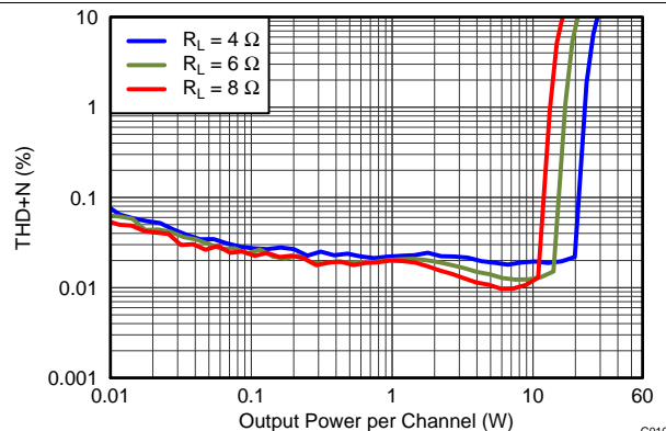
Figure 19. THD+N vs Output Power
