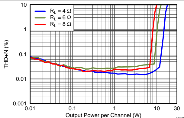
Figure 18. THD+N vs Output Power
