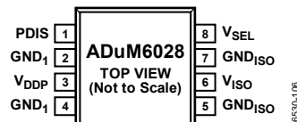
Figure 6. ADuM6028 Pin Configuration
