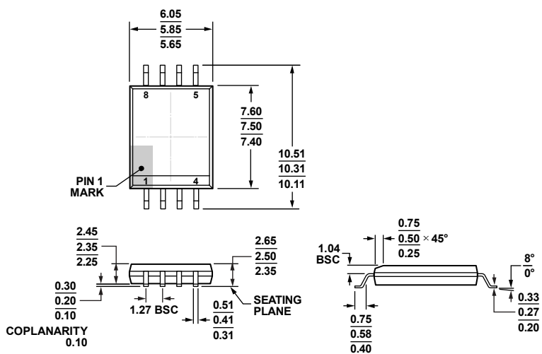
Figure 29. 8-Lead Standard Small Outline Package, with Increased Creepage [SOIC_IC] Wide Body (RI-8-1)
