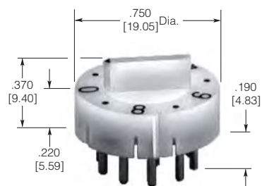
bar type knob Part Number 2-435097-1
