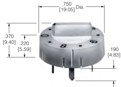
bar type knob Part Number 1-435123-1
