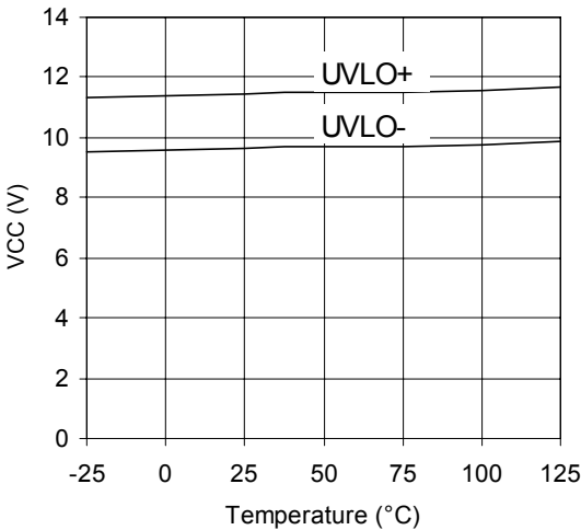
Graph 1. VCCUV+, VCCUV- vs TEMP
