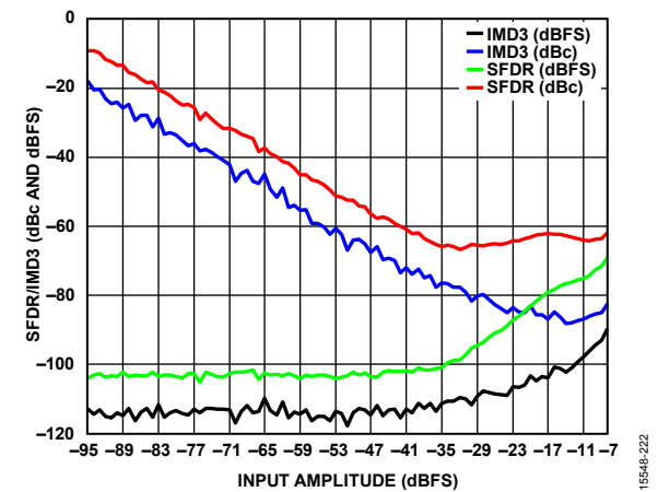
Figure 21. Two-Tone SFDR/IMD3 vs. Input Amplitude with f_{IN1} = 1841.5\text{ MHz} , f_{IN2} = 1846.5\text{ MHz}
