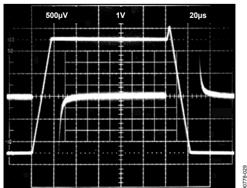
Figure 29. Large Signal Pulse Response and Settling Time, G = -1 ( 0.250 mV = 0.01%), C_L = 100 pF
