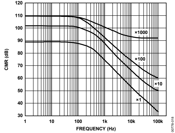
Figure 18. CMR vs. Frequency, ±5 V S
