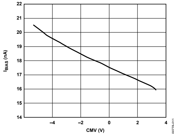
Figure 11. I BIAS vs. CMV, V S = ±5 V
