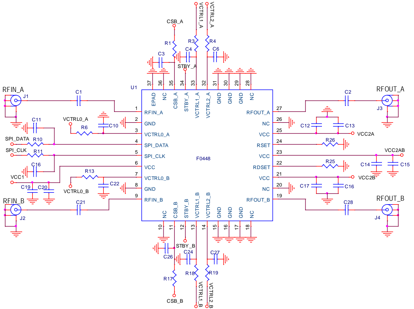
Figure 39. Electrical Schematic
