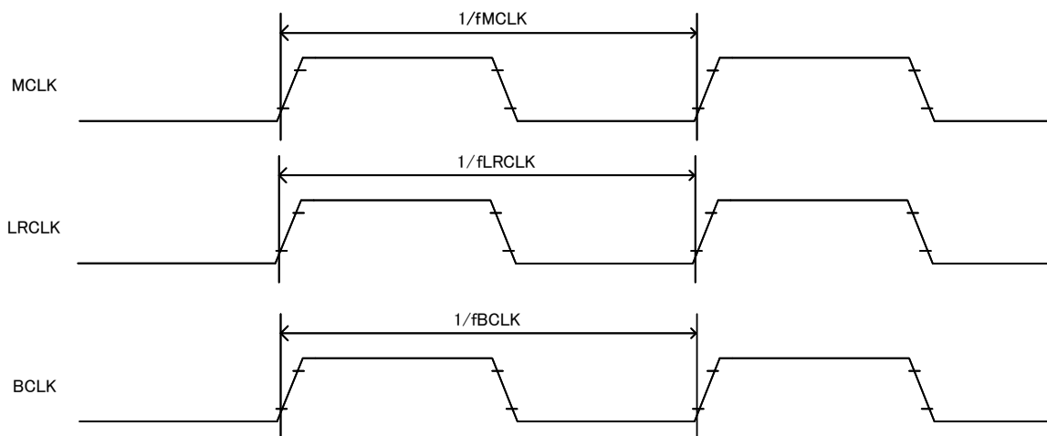
Figure 57. Clock Timing
