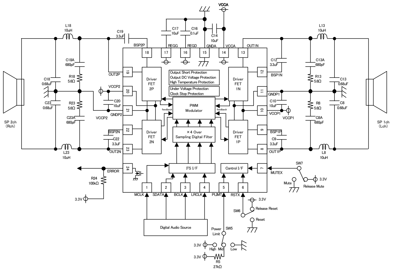
Figure 69. Application Circuit
