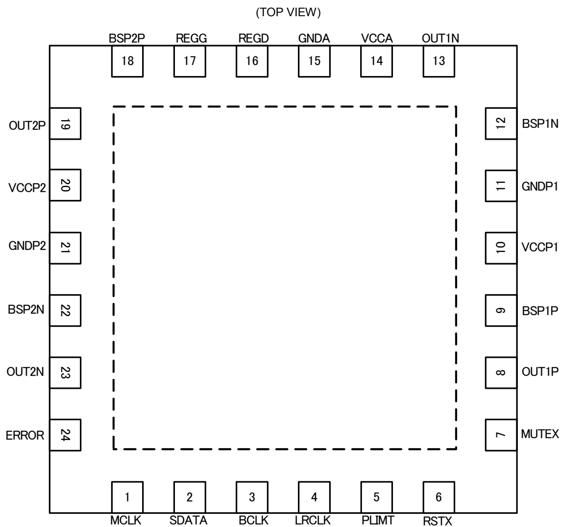
Figure 2. Pin Configuration
