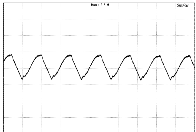
Figure 10: Output Voltage Ripple and Noise at nominal input voltage and max load current (100mV/div, 2us/div) Load cap: 470uF Oscon cap. Bandwidth: 20MHz.
